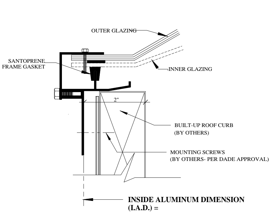
TYPICAL CURB DETAIL
