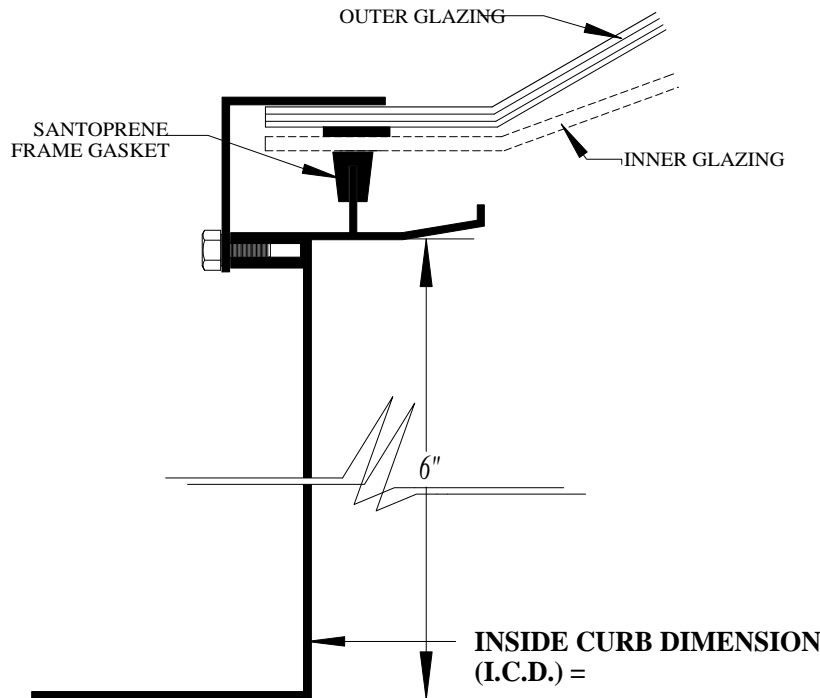
TYPICAL CURB DETAIL
